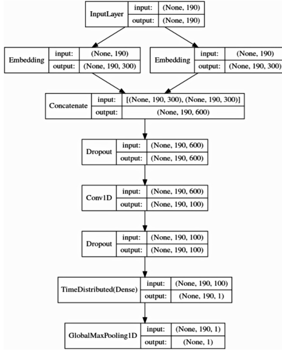
Fig. 1. Description of NNHD.
